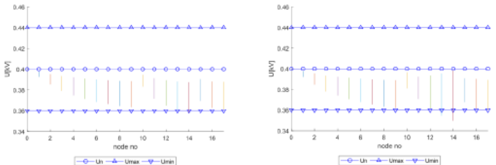
Figure 7: Histogram of node voltages - left without PHEVs, right with PHEVs – Case Two (without electric heating)
