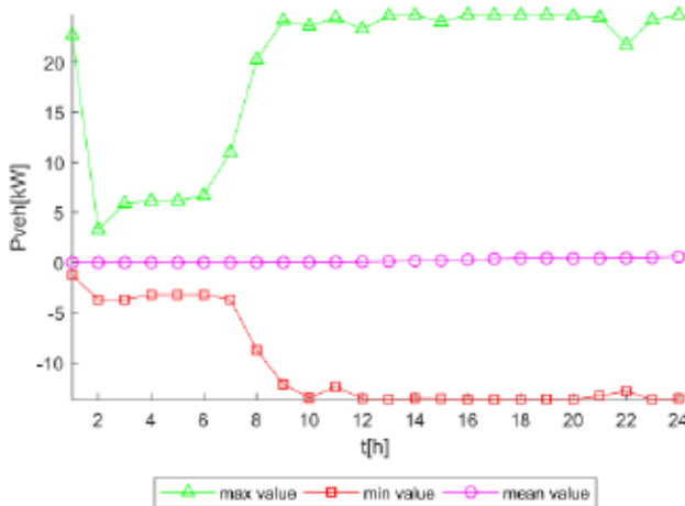
Figure 3: Domain of the generated PHEVs injections
