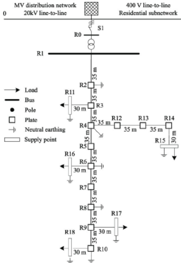
Figure 2: CIGRE Benchmark low voltage grid
