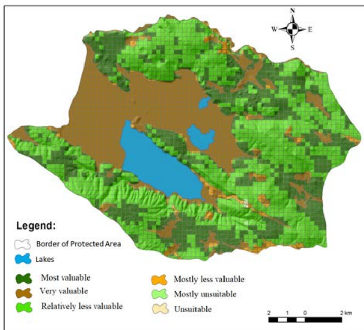
Fig. 3. Geoecological evaluation of Nature Park Hutovo blato.
